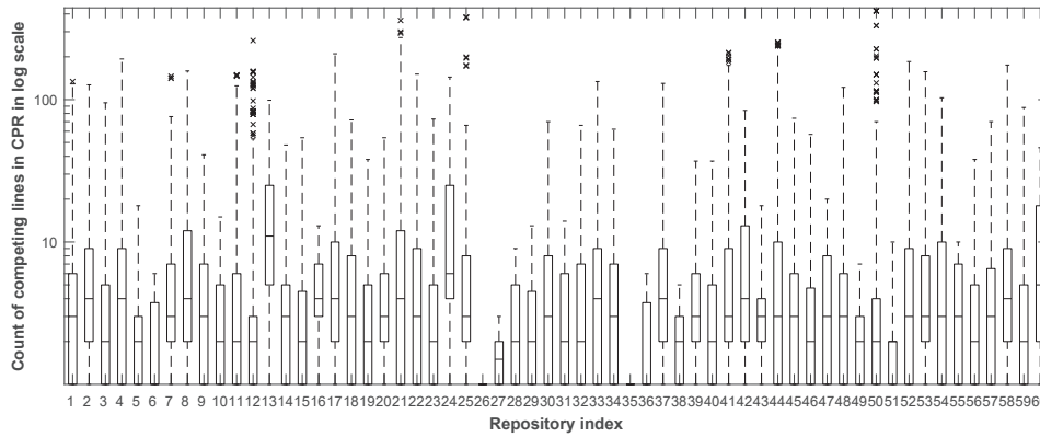
Figure 6. Count of competing lines in competing pull requests in the log scale for each repository.
